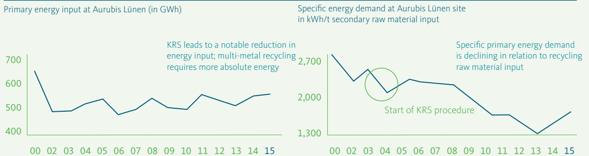
Fig. 2.12: Specific energy demand in relation to recycling raw material input
